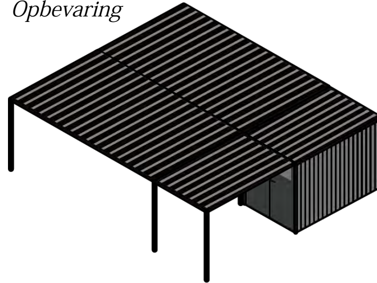
Carport Basic + Carport EXT + Opbevaring + Struktur EXT
